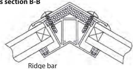
Ridge bar
