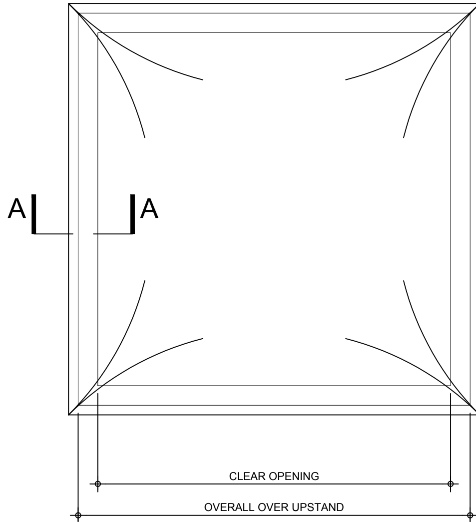
PLAN ON DOUBLE SKIN DOME ROOFLIGHT (1No. REQUIRED AS SHOWN)
